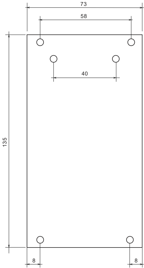
Array Light Enclosure Side Dimensions
